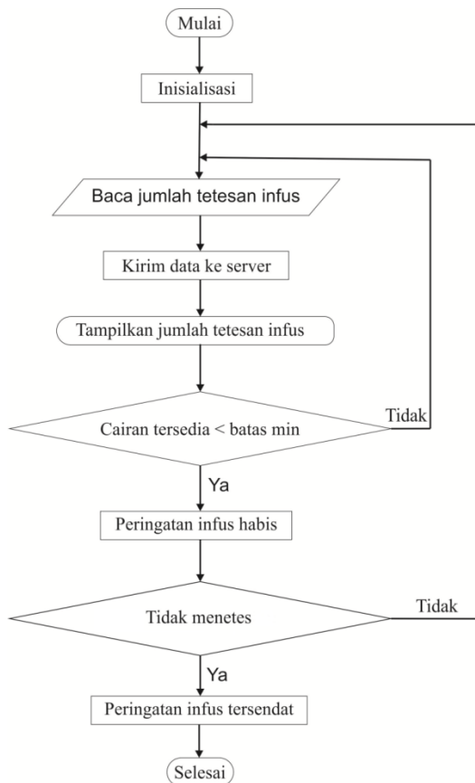
Gambar 4. Flowchart program
