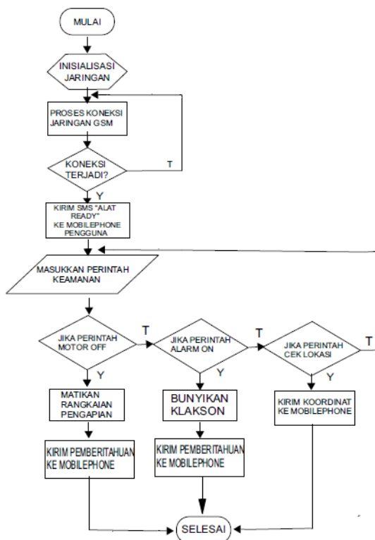
Gambar 4. Flowchart Program
