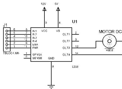
Gambar 5. Rangkaian Driver Motor DC
